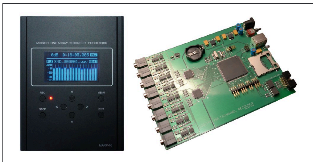
Figure 1. Sixteen-channel microphone array recorder/processor MARP-16
