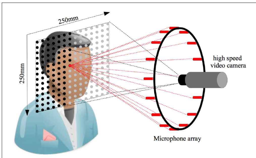
Figure 4. Scanning of the acoustic field distribution (50x50 points) by the circular microphone array
