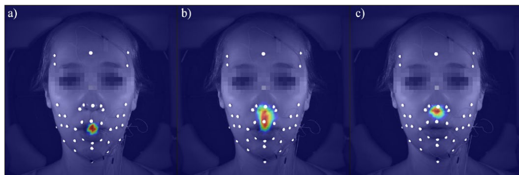
Figure 5. Spatial distribution of the acoustic field synchronised with the image from video camera during realization of nasalized vowel [ɔ̃ʂ] in the word pąsy 'crimsons' in the different articulation phases: a) oral, b) oronasal c) nasal (speaker ZK_f, file 157)
