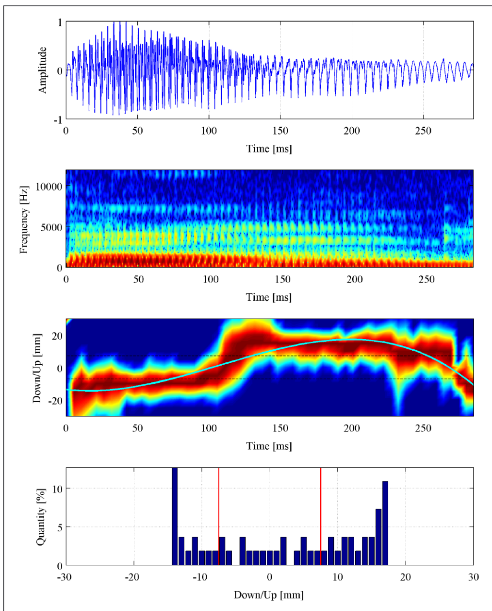
Figure 6. Spatial distribution of the acoustic field correlated with oscillogram, spectrogram, 3rd order polynomial approximation and histogram of realization of nasalized vowel [ɔ̃] in the word pąsy 'crimsons' (speaker ZK_f, file 157)
